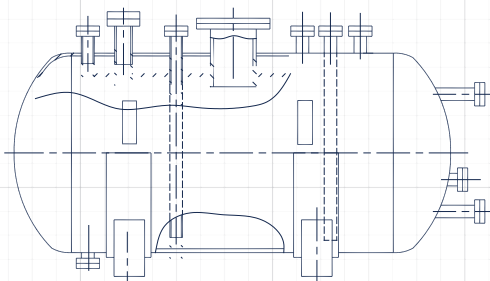
HORIZONTAL WITH ELLIPTICAL BOTTOMS
